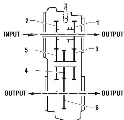
FLOATING GEAR OPPOSITE INPUT SIDE
