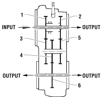
FLOATING GEAR INPUT SIDE
